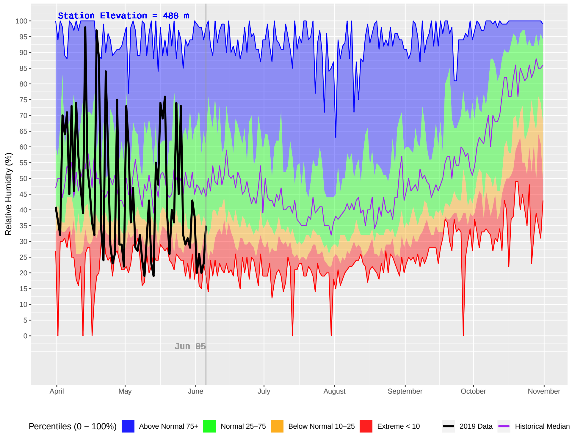
MABEL LAKE 2 (362) : Historical (1987–2018) and Current (2019) Daily Relative Humidity
