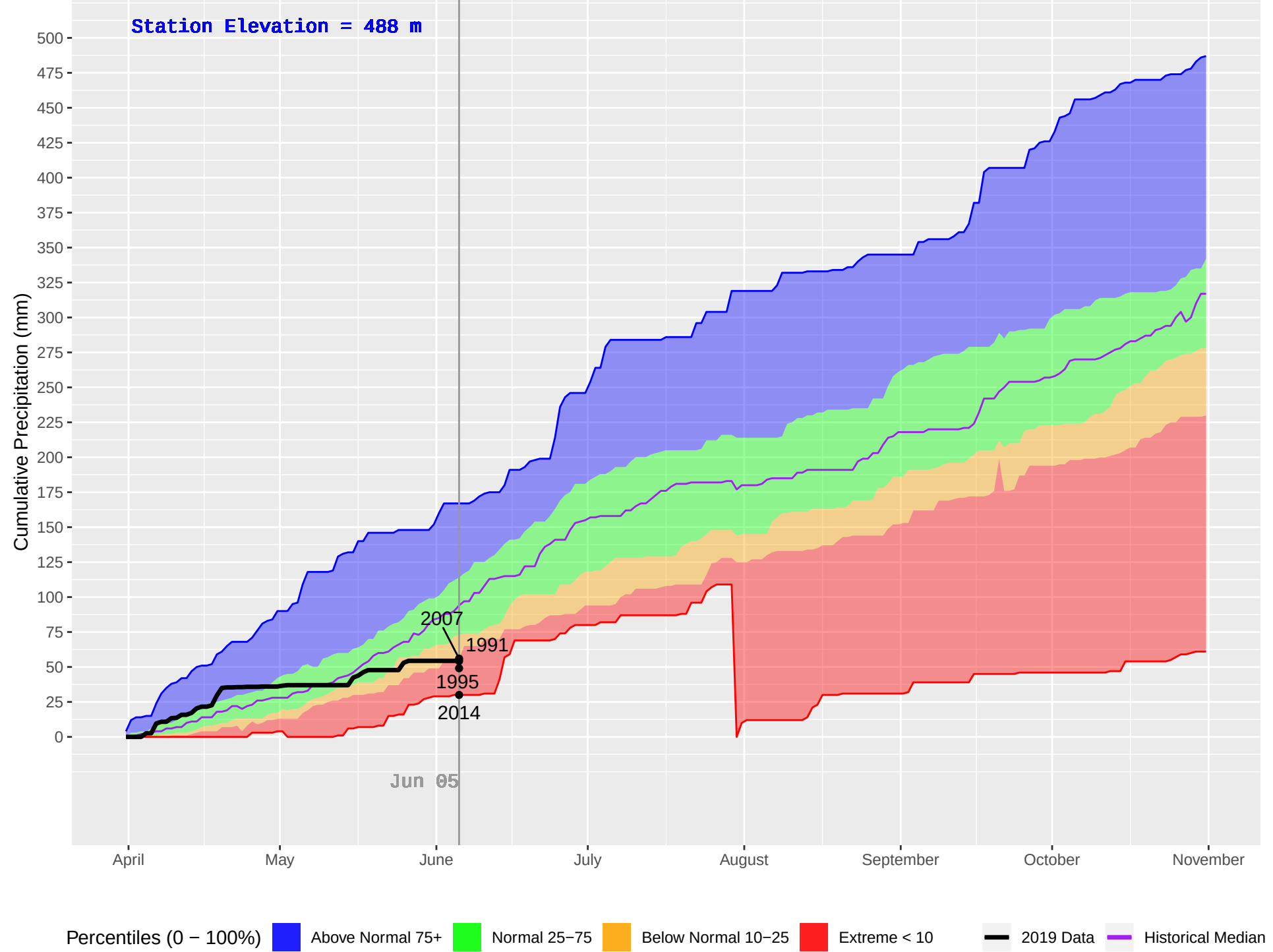
MABEL LAKE 2 (362) : Historical (1987–2018), Current (2019) Daily Cumulative Precipitation
