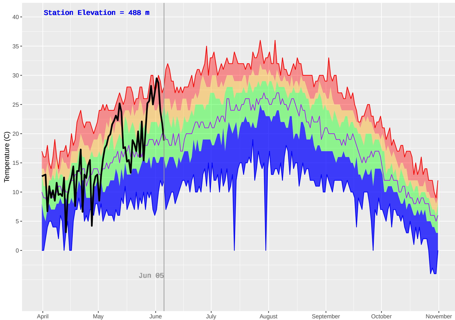
MABEL LAKE 2 (362) : Historical (1987–2018) and Current (2019) Daily Temperature
