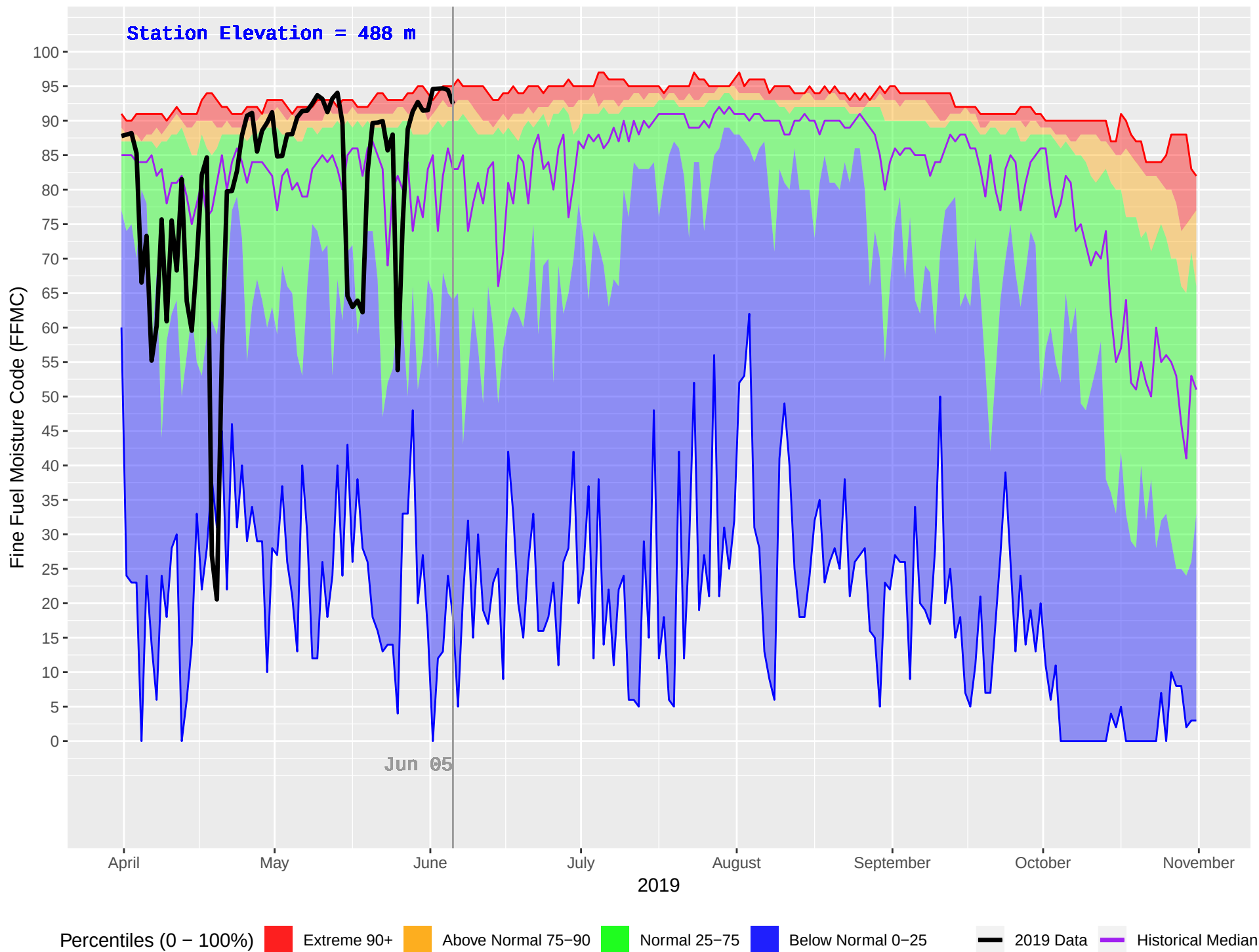
MABEL LAKE 2 (362) : Historical (1987–2018) and Current (2019) Daily Fine Fuel Moisture Code (FFMC)
