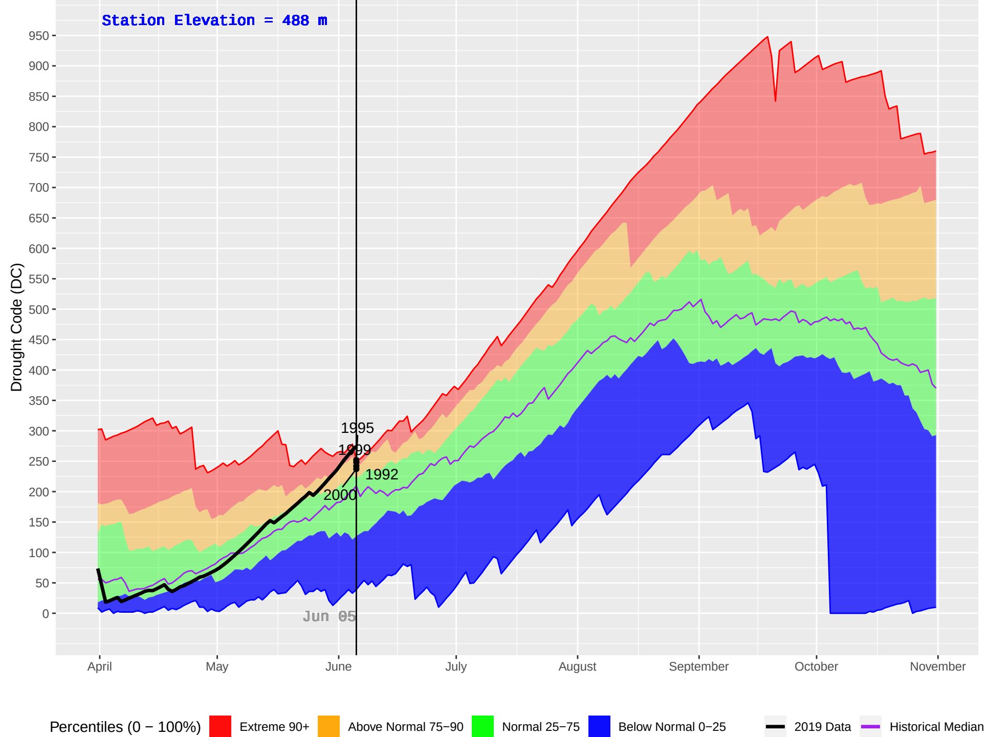
MABEL LAKE 2 (362) : Historical (1987–2018) and Current (2019) Daily Drought Code (DC)
