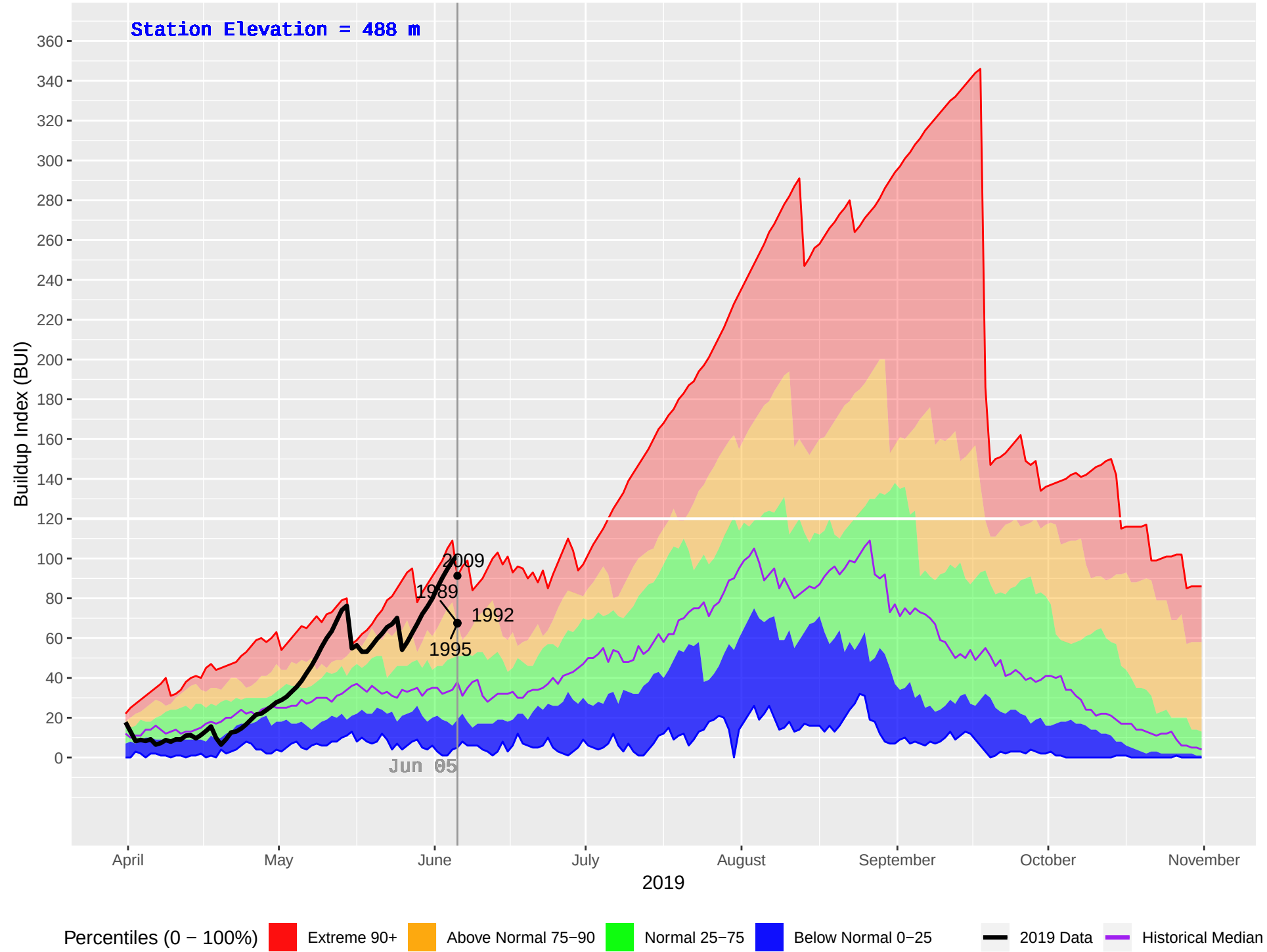
MABEL LAKE 2 (362) : Historical (1987–2018), Current (2019) Daily Buildup Index (BUI)
