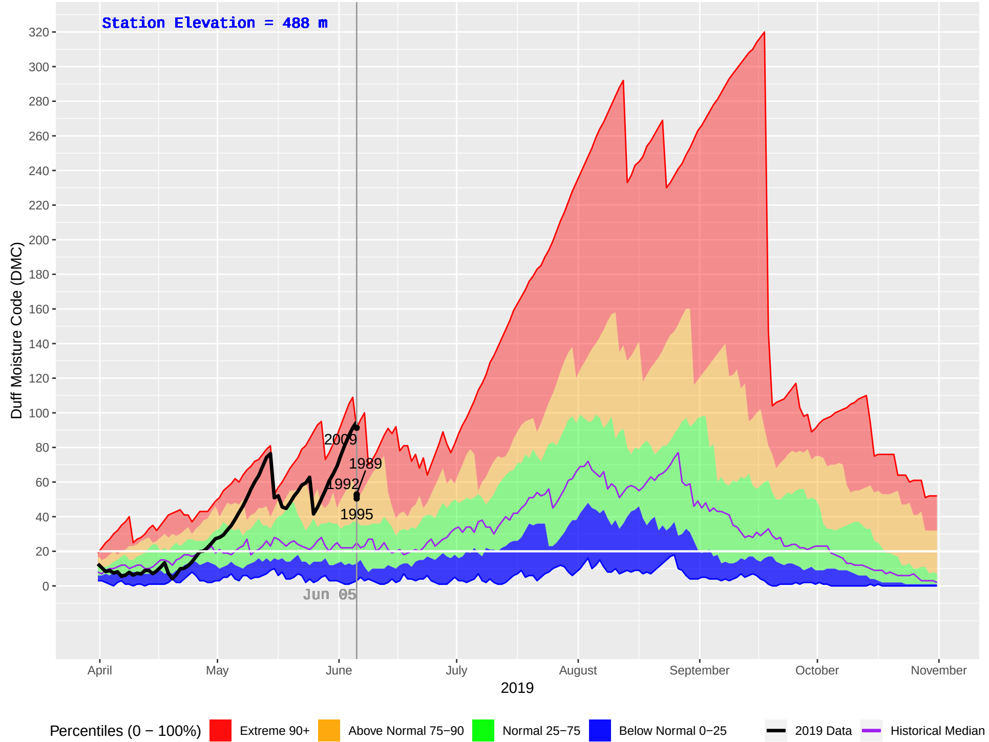
MABEL LAKE 2 (362) : Historical (1987–2018), Current (2019) Daily Duff Moisture Code (DMC)
